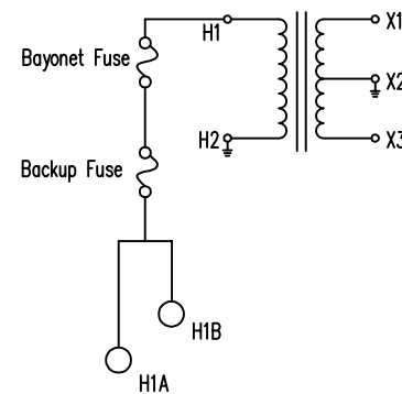
Connection Diagram
